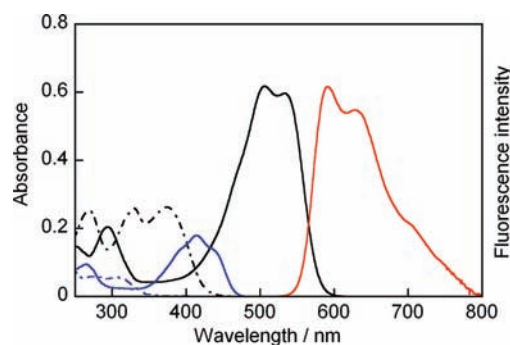
Figure 2. Absorption spectra of 8a (black dashed line), 8b (black solid line), and photostationary state under irradiation with 365 nm light in 1,4-dioxane ( 1.0 \times 10^{-5} M) and fluorescence spectrum of 8b (red solid line) under irradiation with 532 nm light. The photostationary spectrum overlaps with the spectrum of 8b . The absorption spectra of 2a (blue dashed line) and 2b (blue solid line) in 1,4-dioxane ( 1.0 \times 10^{-5} M) were also shown as a reference.
